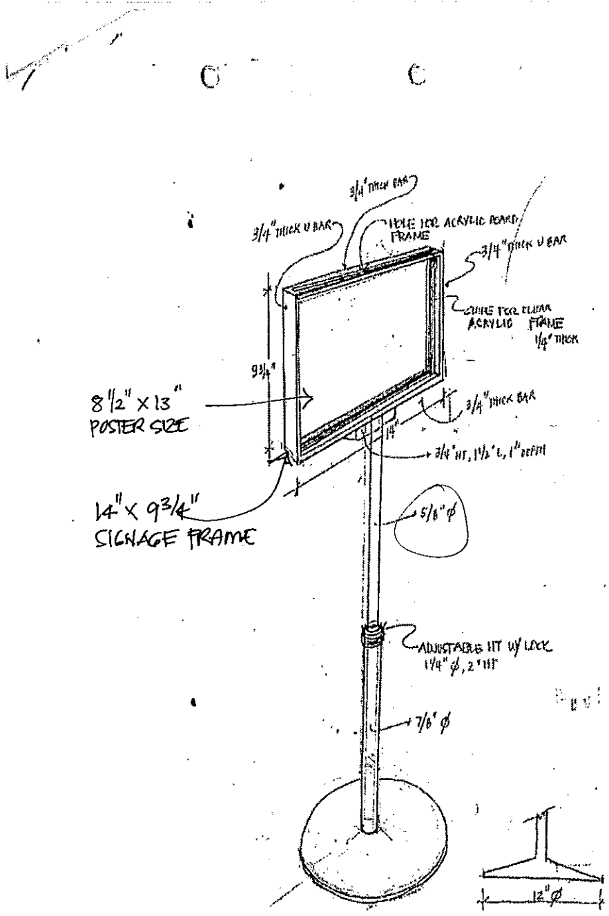
○ SIGN STAND (STAINLESS) HEIGHT: MINIMUM OF 3 1/2 FT MAXIMUM OF 6 FT (8 FT HT) (STOP DRAWING)
